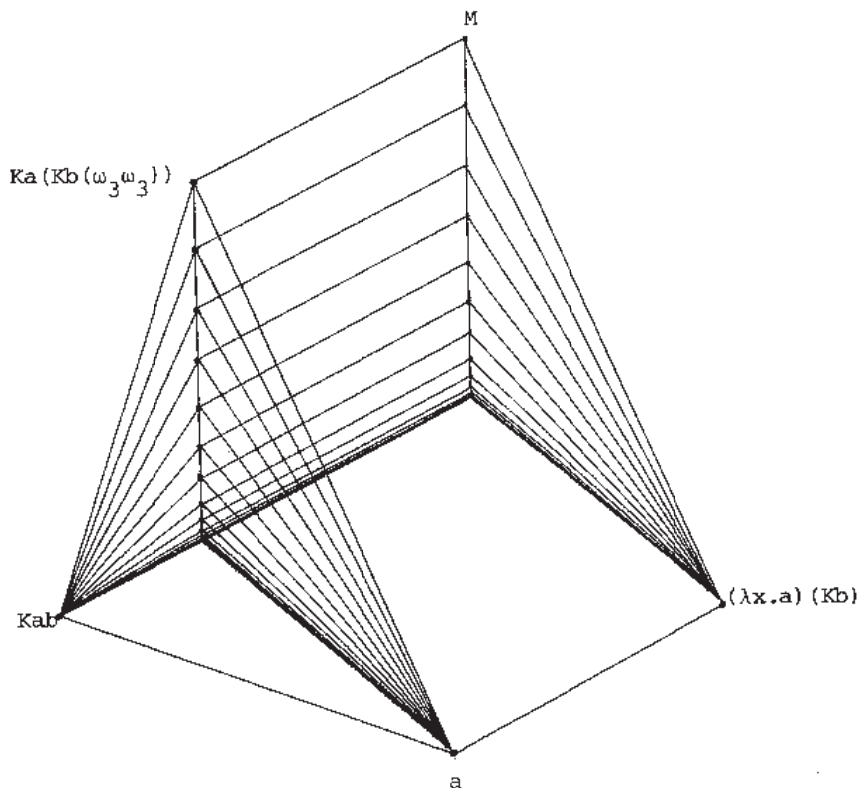
Reduction graph of M \equiv (\lambda x. \text{Ka}(x(\omega_3 \omega_3)))(\text{Kb}) .
